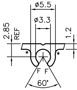
DETAIL OF B SCALE 2:1
