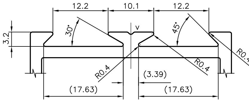
DETAIL-A
