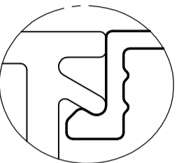
DETAIL-C SCALE:-3:1
