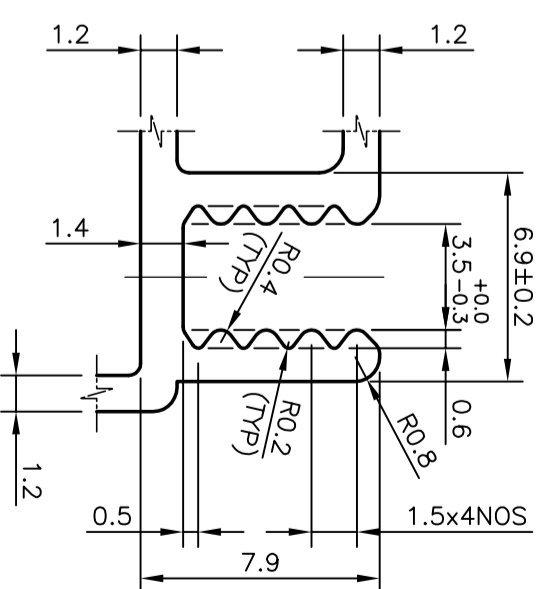
DETAIL OF "A" SCALE 4:1
